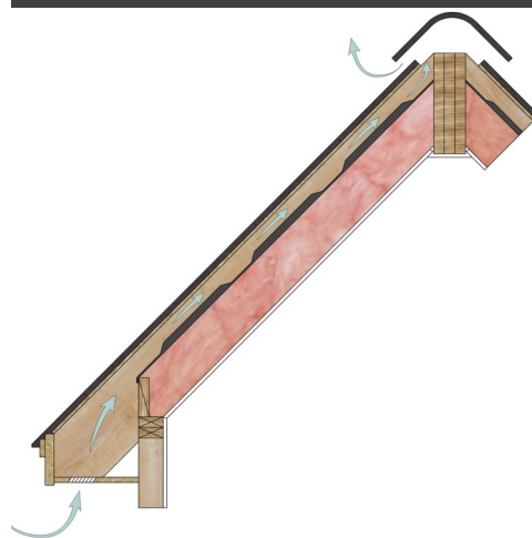
Figure 2. Vented Roof Assembly
