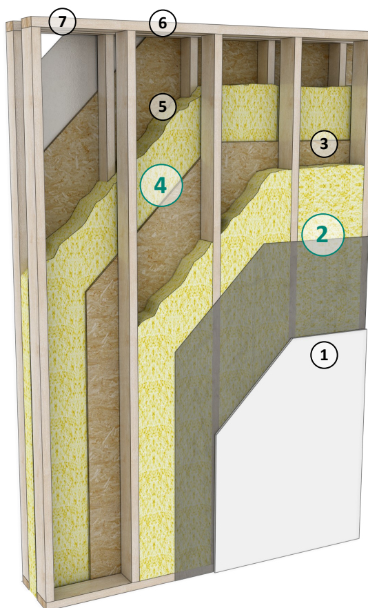
Figure 6. Double Wall Construction
